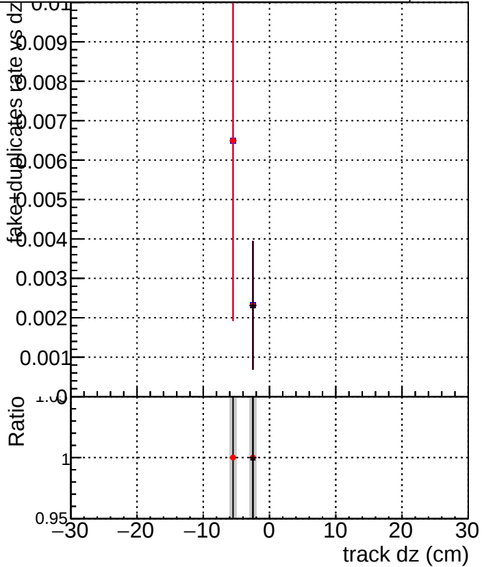
DQM_original_step2_pt1to20_eta1p0to1p4 DQM_mkFit_step2_pt1to20_eta1p0to1p4 DQM_pixelCPETemplate_step2_pt1to20_eta1p0to1p4
