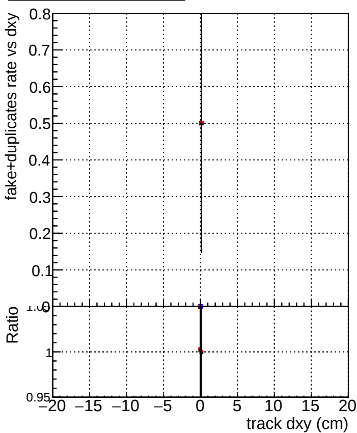
DQM_original_step2_pt1to20_eta1p0to1p4 DQM_mkFit_step2_pt1to20_eta1p0to1p4 DQM_pixelCPETemplate_step2_pt1to20_eta1p0to1p4
