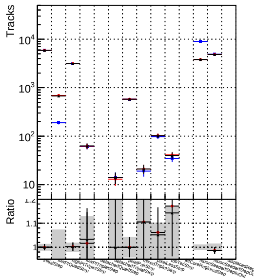
Number of tracks vs collection Legend: DQM_original_step2_pt1to20_eta1p0to1p4 DQM_mkFit_step2_pt1to20_eta1p0to1p4 DQM_pixelCPETemplate_step2_pt1to20_eta1p0to1p4
