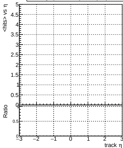
— DQM_original_step2_pt1to20_eta1p0to1p4 — DQM_mkFit_step2_pt1to20_eta1p0to1p4 — DQM_pixelCPETemplate_step2_pt1to20_eta1p0to1p4
