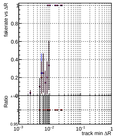
DQM_original_step2_pt1to20_eta0p4to1p0 DQM_mkFit_step2_pt1to20_eta0p4to1p0 DQM_pixelCPETemplate_step2_pt1to20_eta0p4to1p0
