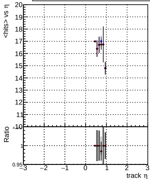
— DQM_original_step2_pt1to20_eta0p4to1p0 — DQM_mkFit_step2_pt1to20_eta0p4to1p0 — DQM_pixelCPETemplate_step2_pt1to20_eta0p4to1p0
