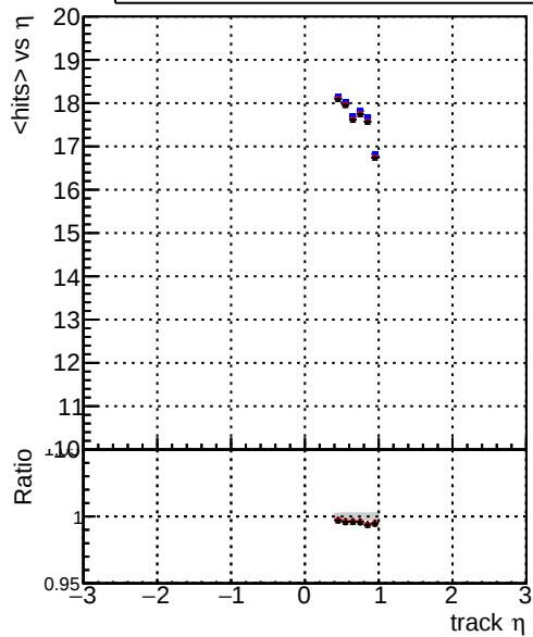
mean hits vs \eta — DQM_original_step2_pt1to20_eta0p4to1p0 — DQM_mkFit_step2_pt1to20_eta0p4to1p0 — DQM_pixelCPETemplate_step2_pt1to20_eta0p4to1p0
