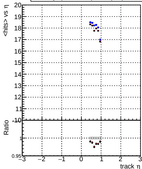
mean hits — DQM_original_step2_pt1to20_eta0p4to1p0 — DQM_mkFit_step2_pt1to20_eta0p4to1p0 — DQM_pixelCPETemplate_step2_pt1to20_eta0p4to1p0
