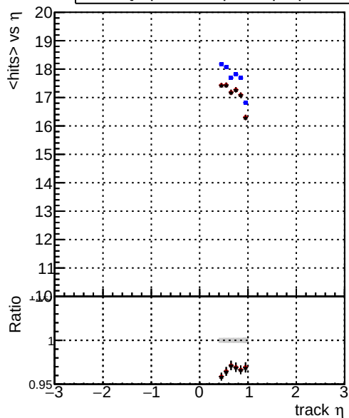
mean hit — DQM_original_step2_pt1to20_eta0p4to1p0 — DQM_mkFit_step2_pt1to20_eta0p4to1p0 — DQM_pixelCPEtemplate_step2_pt1to20_eta0p4to1p0
