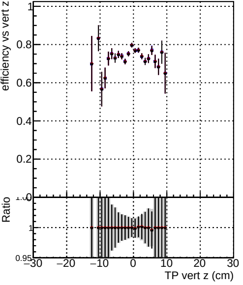
Efficiency vs TP vert z Legend: DQM_original_step2_pt1to20_eta0p4to1p0 DQM_mkFit_step2_pt1to20_eta0p4to1p0 DQM_pixelCPETemplate_step2_pt1to20_eta0p4to1p0
