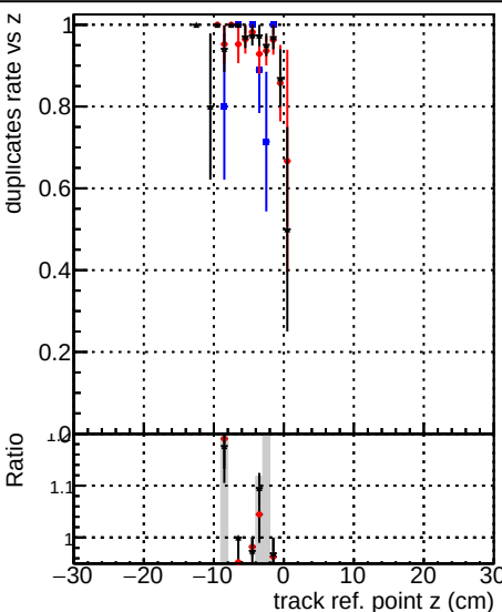
—■— DQM_original_step2_pt1to1000_eta2p6to4p0 —●— DQM_mkFit_step2_pt1to1000_eta2p6to4p0 —×— DQM_pixelCPETemplate_step2_pt1to1000_eta2p6to4p0
