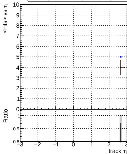
mean hit — DQM_original_step2_pt1to1000_eta2p6to4p0 — DQM_mkFit_step2_pt1to1000_eta2p6to4p0 — DQM_pixelCPEtemplate_step2_pt1to1000_eta2p6to4p0
