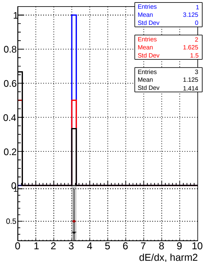
—■— DQM_original_step2_pt1to1000_eta2p6to4p0 —●— DQM_mkFit_step2_pt1to1000_eta2p6to4p0 —▲— DQM_pixelCPETemplate_step2_pt1to1000_eta2p6to4p0
