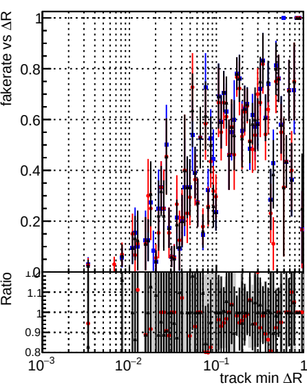
Legend: DQM original step2 pt1to1000 eta2p0to2p5 (blue), DQM mkFit step2 pt1to1000 eta2p0to2p5 (red), DQM pixelCPETemplate step2 pt1to1000 eta2p0to2p5 (black)
