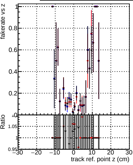
—•— DQM_original_step2_pt1to1000_eta2p0to2p5 —•— DQM_mkFit_step2_pt1to1000_eta2p0to2p5 —•— DQM_pixelCPETemplate_step2_pt1to1000_eta2p0to2p5
