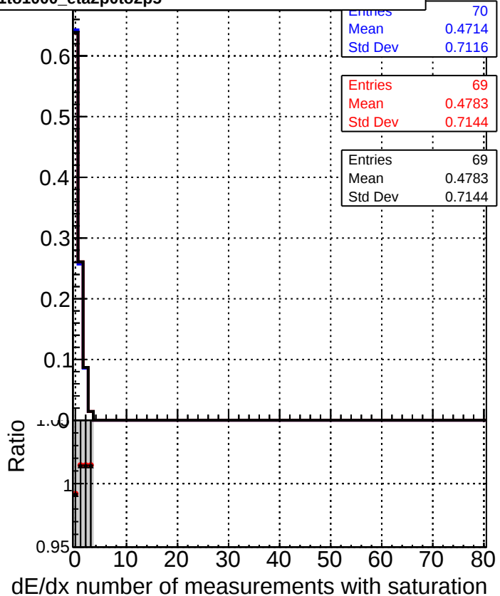
—■— DQM_original_step2_pt1to1000_eta2p0to2p5 —●— DQM_mkFit_step2_pt1to1000_eta2p0to2p5 —▲— DQM_pixelCPETemplate_step2_pt1to1000_eta2p0to2p5
