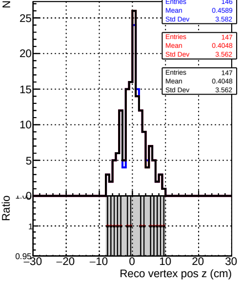
Recons Legend: DQM_original_step2_pt1to1000_eta2p0to2p5 (blue line) DQM_mkFit_step2_pt1to1000_eta2p0to2p5 (red line) DQM_pixelCPETemplate_step2_pt1to1000_eta2p0to2p5 (black line)
