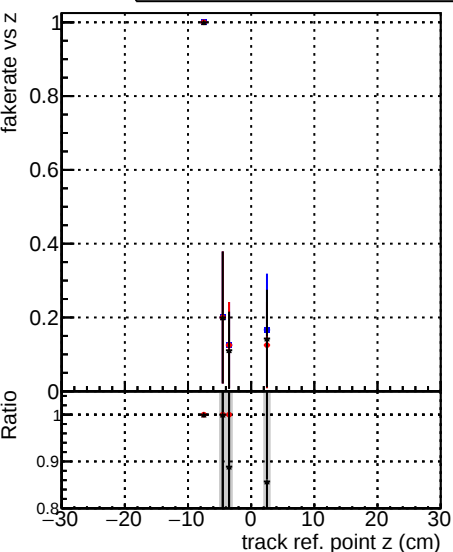
Fake rate vs v DQM_original_step2_pt1to1000_eta2p0to2p5 DQM_mkFit_step2_pt1to1000_eta2p0to2p5 DQM_pixelCPETemplate_step2_pt1to1000_eta2p0to2p5
