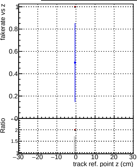
Fake rate vs v DOM original step2_pt1to1000_eta2p0to2p5 DOM mkFit step2_pt1to1000_eta2p0to2p5 DOM_pixelCPETemplate step2_pt1to1000_eta2p0to2p5
