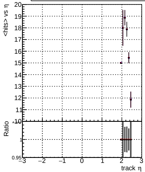
mean hit — DQM_original_step2_pt1to1000_eta2p0to2p5 — DQM_mkFit_step2_pt1to1000_eta2p0to2p5 — DQM_pixelCPEtemplate_step2_pt1to1000_eta2p0to2p5
