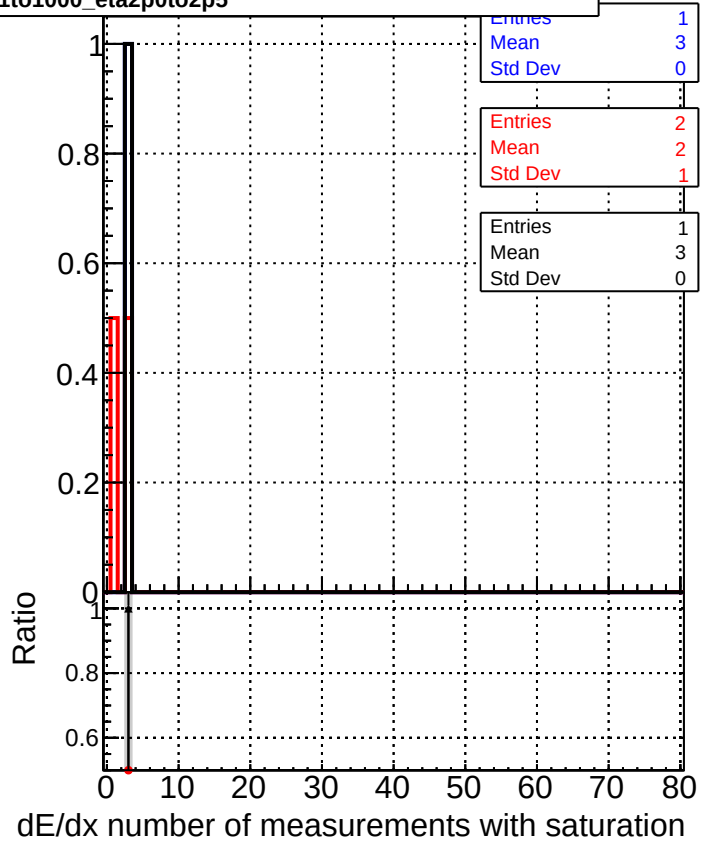
— DQM_original_step2_pt1to1000_eta2p0to2p5 — DQM_mkFit_step2_pt1to1000_eta2p0to2p5 — DQM_pixelCPETemplate_step2_pt1to1000_eta2p0to2p5
