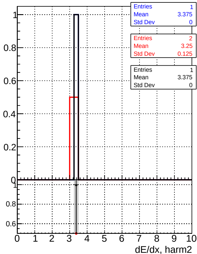
— DQM_original_step2_pt1to1000_eta2p0to2p5 — DQM_mkFit_step2_pt1to1000_eta2p0to2p5 — DQM_pixelCPETemplate_step2_pt1to1000_eta2p0to2p5
