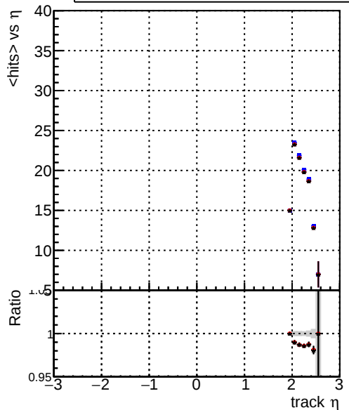
mean hits — DQM_original_step2_pt1to1000_eta2p0to2p5 — DQM_mkFit_step2_pt1to1000_eta2p0to2p5 — DQM_pixelCPEtemplate_step2_pt1to1000_eta2p0to2p5
