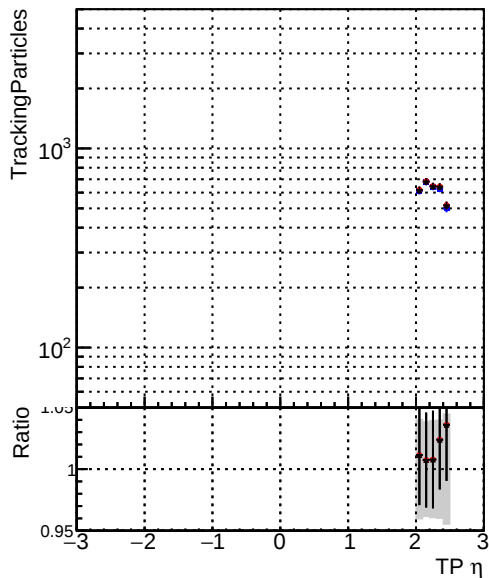
—•— DQM_original_step2_pt1to1000_eta2p0to2p5 —•— DQM_mkFit_step2_pt1to1000_eta2p0to2p5 —•— DQM_pixelCPETemplate_step2_pt1to1000_eta2p0to2p5
