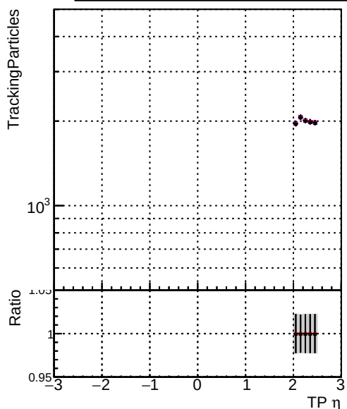
Legend: - DQM_original_step2_pt1to1000_eta2p0to2p5 (blue line with dots) - DQM_mkFit_step2_pt1to1000_eta2p0to2p5 (red line with dots) - DQM_pixelCPETemplate_step2_pt1to1000_eta2p0to2p5 (black line with dots)
