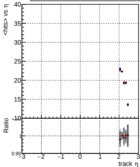
mean hits — DQM_original_step2_pt1to1000_eta2p0to2p5 — DQM_mkFit_step2_pt1to1000_eta2p0to2p5 — DQM_pixelCPETemplate_step2_pt1to1000_eta2p0to2p5
