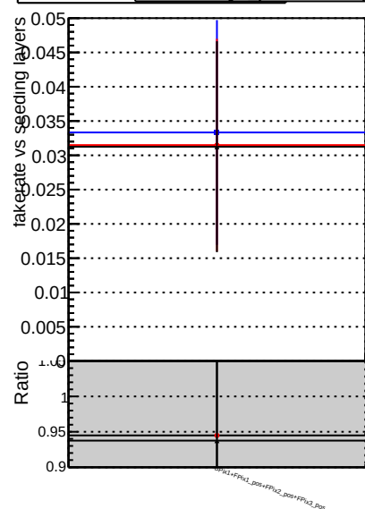
Fake rate vs. DOM original step2 pt1to1000 eta2p0to2p5 DOM min step2 pt1to1000 eta2p0to2p5 DOM pixelCPE template step2 pt1to1000 eta2p0to2p5
