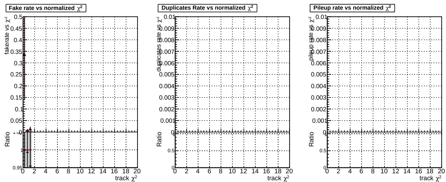
Fake rate vs. DOM original step2 pt1to1000 eta2p0to2p5 DOM min step2 pt1to1000 eta2p0to2p5 DOM pixelCPE template step2 pt1to1000 eta2p0to2p5
