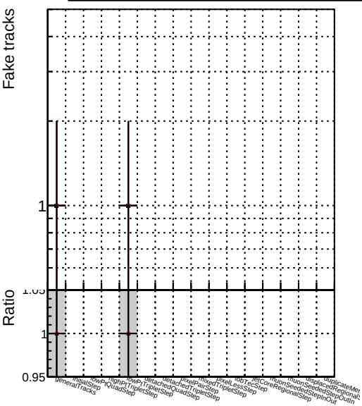
Number —●— DQM_mkFit_step2_pt1to1000_eta1p6to2p0 —▲— DQM_pixelCPETemplate_step2_pt1to1000_eta1p6to2p0
