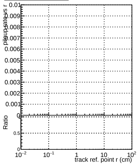
—•— DQM_original_step2_pt1to1000_eta1p6to2p0 —•— DQM_mkFit_step2_pt1to1000_eta1p6to2p0 —•— DQM_pixelCPETemplate_step2_pt1to1000_eta1p6to2p0
