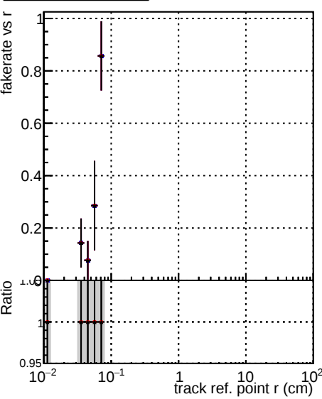
—•— DQM_original_step2_pt1to1000_eta1p6to2p0 —•— DQM_mkFit_step2_pt1to1000_eta1p6to2p0 —•— DQM_pixelCPETemplate_step2_pt1to1000_eta1p6to2p0
