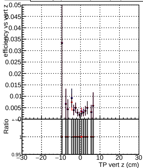
Efficiency vs. sim PV z —●— DQM_original_step2_pt1to1000_eta1p6to2p0 —●— DQM_mkFit_step2_pt1to1000_eta1p6to2p0 —●— DQM_pixelCPETemplate_step2_pt1to1000_eta1p6to2p0
