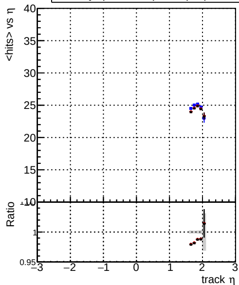
mean hits vs \eta — DQM_original_step2_pt1to1000_eta1p6to2p0 — DQM_mkFit_step2_pt1to1000_eta1p6to2p0 — DQM_pixelCPETemplate_step2_pt1to1000_eta1p6to2p0
