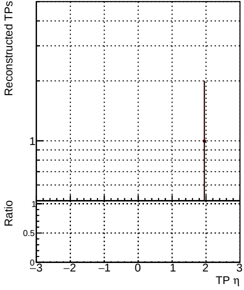
Legend: - DQM_original_step2_pt1to1000_eta1p6to2p0 - DQM_mkFit_step2_pt1to1000_eta1p6to2p0 - DQM_pixelCPETemplate_step2_pt1to1000_eta1p6to2p0
