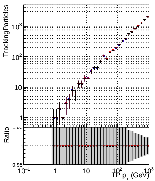
Legend: - DQM_original_step2_pt1to1000_eta1p6to2p0 - DQM_mkFit_step2_pt1to1000_eta1p6to2p0 - DQM_pixelCPETemplate_step2_pt1to1000_eta1p6to2p0
