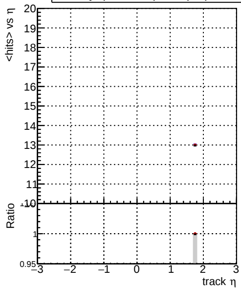
mean hit DQM_original_step2_pt1to1000_eta1p6to2p0 DQM_mkFit_step2_pt1to1000_eta1p6to2p0 DQM_pixelCPETemplate_step2_pt1to1000_eta1p6to2p0
