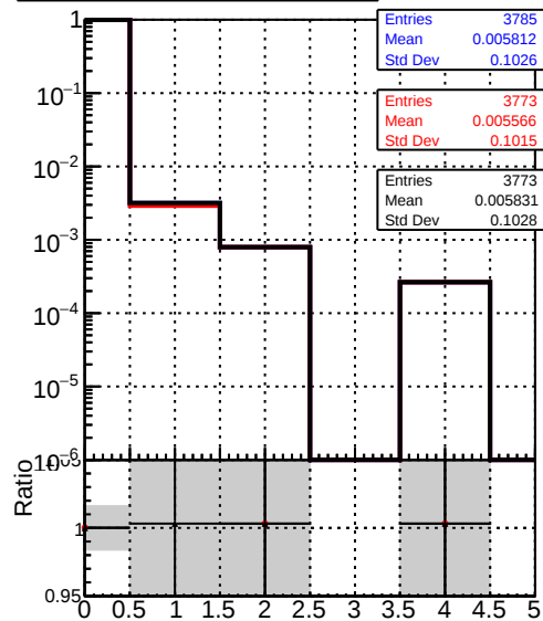
mean hit — DQM_original_step2_pt1to1000_eta1p6to2p0 — DQM_mkFit_step2_pt1to1000_eta1p6to2p0 — DQM_pixelCPETemplate_step2_pt1to1000_eta1p6to2p0
