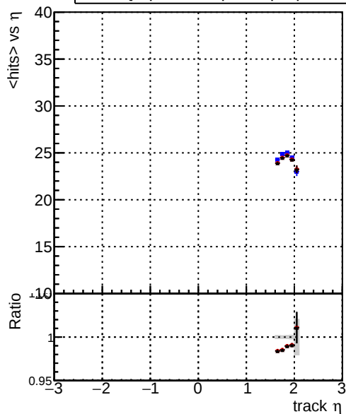
mean hits — DQM_original_step2_pt1to1000_eta1p6to2p0 — DQM_mkFit_step2_pt1to1000_eta1p6to2p0 — DQM_pixelCPEtemplate_step2_pt1to1000_eta1p6to2p0
