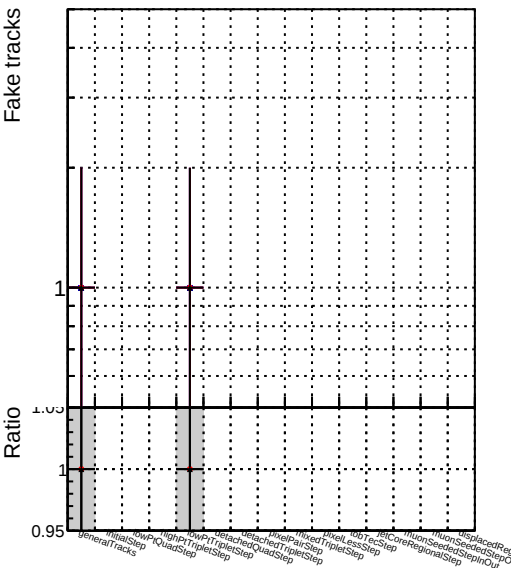
Number Legend 1 DQM_mkFit_step2__pt1to1000_eta1p6to2p0 2 DQM_pixelCPETemplate_step2__pt1to1000_eta1p6to2p0
