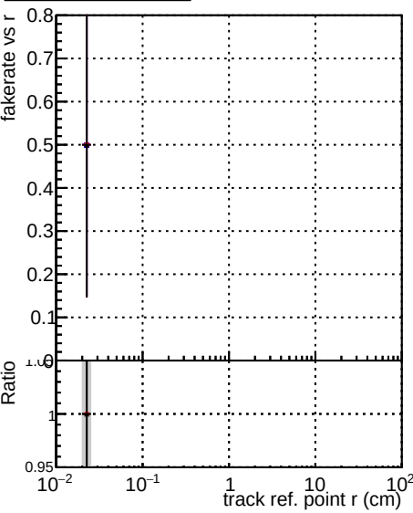
Fake rate vs verpos DQM original step2_pt1to1000_eta1p6to2p0 DQM mkFit step2_pt1to1000_eta1p6to2p0 DQM_pixelCPETemplate step2_pt1to1000_eta1p6to2p0
