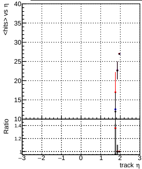
DQM_original_step2_pt1to1000_eta1p6to2p0 DQM_mkFit_step2_pt1to1000_eta1p6to2p0 DQM_pixelCPETemplate_step2_pt1to1000_eta1p6to2p0
