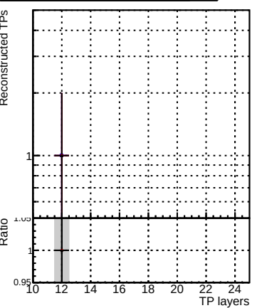
N of sim Legend: DQM_original_step2_pt1to1000_eta1p4to1p6 DQM_mkFit_step2_pt1to1000_eta1p4to1p6 DQM_pixelCPETemplate_step2_pt1to1000_eta1p4to1p6
