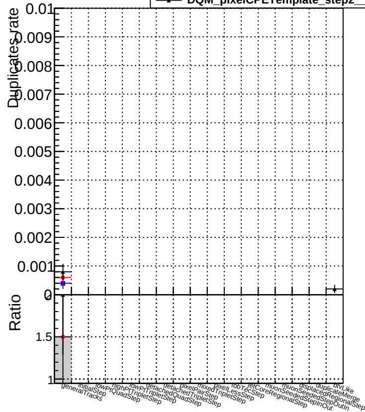
—●— DQM_mkFit_step2_pt1to1000_eta1p4to1p6 —▲— DQM_pixelCPETemplate_step2_pt1to1000_eta1p4to1p6
