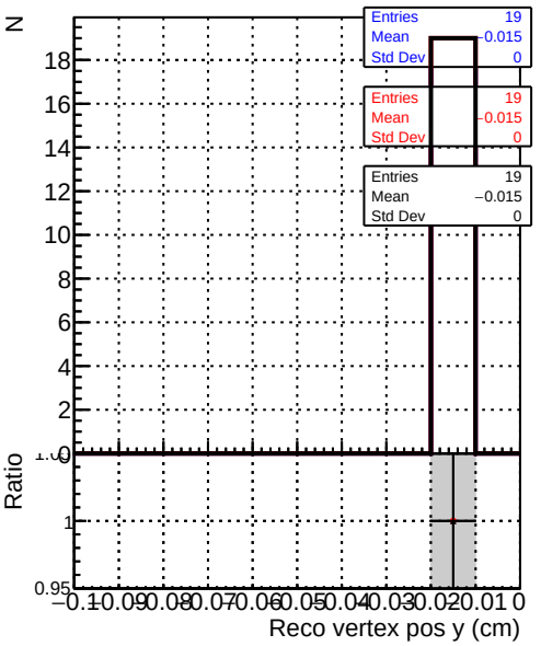
Recons Legend: — DQM_original_step2_pt1to1000_eta1p4to1p6 (blue) — DQM_mkFit_step2_pt1to1000_eta1p4to1p6 (red) — DQM_pixelCPETemplate_step2_pt1to1000_eta1p4to1p6 (black)
