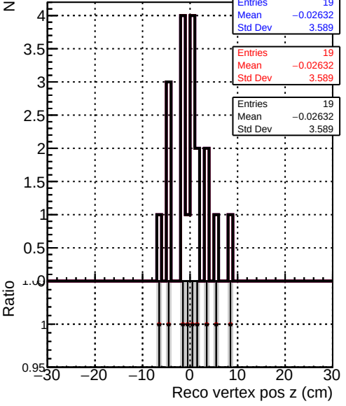
Recons Legend: — DQM_original_step2_pt1to1000_eta1p4to1p6 (blue) — DQM_mkFit_step2_pt1to1000_eta1p4to1p6 (red) — DQM_pixelCPETemplate_step2_pt1to1000_eta1p4to1p6 (black)
