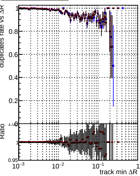
Legend: - DQM_original_step2_pt1to1000_eta1p4to1p6 (blue line with dots) - DQM_mkFit_step2_pt1to1000_eta1p4to1p6 (red line with dots) - DQM_pixelCPETemplate_step2_pt1to1000_eta1p4to1p6 (black line with dots)
