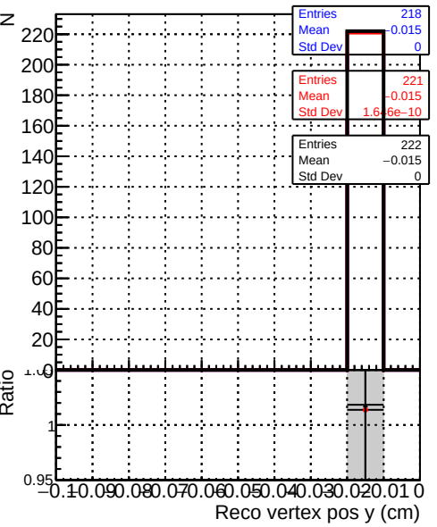
Recons Legend: DQM_original_step2_pt1to1000_eta1p4to1p6 DQM_mkFit_step2_pt1to1000_eta1p4to1p6 DQM_pixelCPETemplate_step2_pt1to1000_eta1p4to1p6
