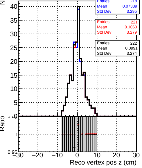
Recons Legend: DQM_original_step2_pt1to1000_eta1p4to1p6 DQM_mkFit_step2_pt1to1000_eta1p4to1p6 DQM_pixelCPETemplate_step2_pt1to1000_eta1p4to1p6
