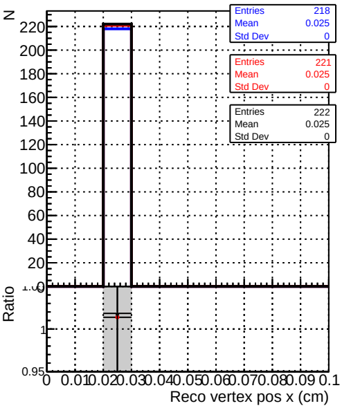
Recons Legend: DQM_original_step2_pt1to1000_eta1p4to1p6 DQM_mkFit_step2_pt1to1000_eta1p4to1p6 DQM_pixelCPETemplate_step2_pt1to1000_eta1p4to1p6
