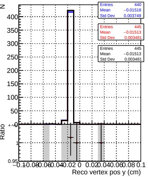
Recons Legend: DQM_original_step2_pt1to1000_eta1p4to1p6 (blue line) DQM_mkFit_step2_pt1to1000_eta1p4to1p6 (red line) DQM_pixelCPETemplate_step2_pt1to1000_eta1p4to1p6 (black line)
