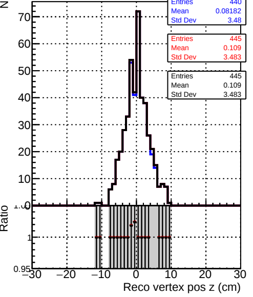
Recons Legend: DQM_original_step2_pt1to1000_eta1p4to1p6 (blue line) DQM_mkFit_step2_pt1to1000_eta1p4to1p6 (red line) DQM_pixelCPETemplate_step2_pt1to1000_eta1p4to1p6 (black line)
