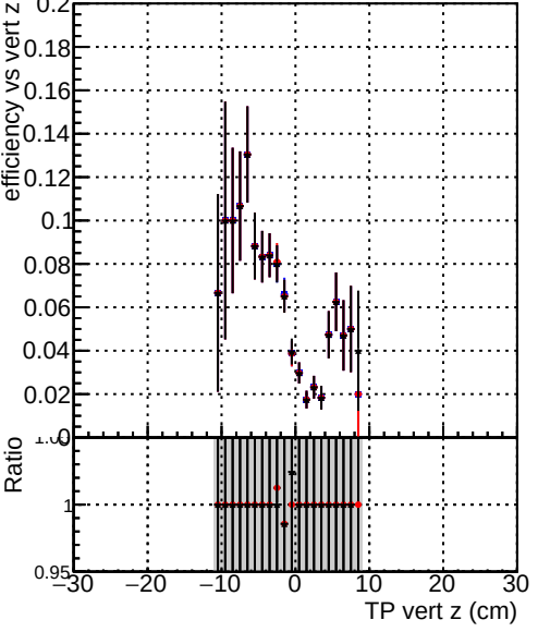
Efficiency vs TP vert z (cm) Legend: DQM_original_step2_pt1to1000_eta1p4to1p6 DQM_mkFit_step2_pt1to1000_eta1p4to1p6 DQM_pixelCPETemplate_step2_pt1to1000_eta1p4to1p6
