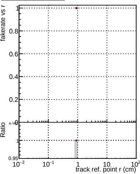
Legend: - DQM_original_step2_pt1to1000_eta1p4to1p6 (blue line with dots) - DQM_mkFit_step2_pt1to1000_eta1p4to1p6 (red line with dots) - DQM_pixelCPETemplate_step2_pt1to1000_eta1p4to1p6 (grey line with dots)
