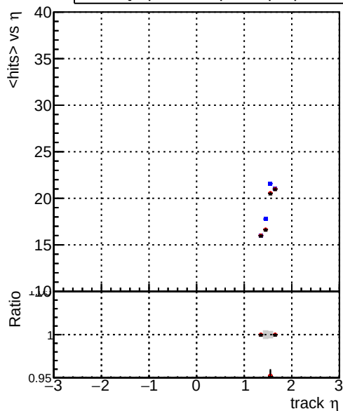
mean hits vs \eta — DQM_original_step2_pt1to1000_eta1p4to1p6 — DQM_mkFit_step2_pt1to1000_eta1p4to1p6 — DQM_pixelCPETemplate_step2_pt1to1000_eta1p4to1p6
