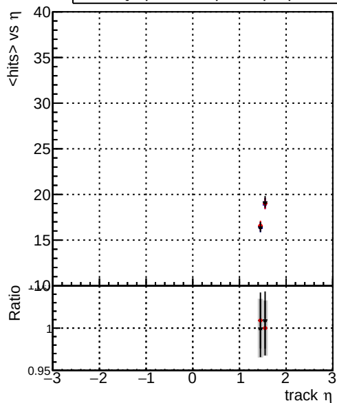
mean hits vs \eta DQM_original_step2_pt1to1000_eta1p4to1p6 DQM_mkFit_step2_pt1to1000_eta1p4to1p6 DQM_pixelCPETemplate_step2_pt1to1000_eta1p4to1p6
