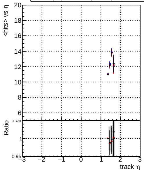
mean hits vs \eta — DQM_original_step2_pt1to1000_eta1p4to1p6 — DQM_mkFit_step2_pt1to1000_eta1p4to1p6 — DQM_pixelCPEtemplate_step2_pt1to1000_eta1p4to1p6
