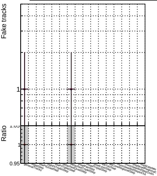
Number —●— DQM_mkFit_step2_pt1to1000_eta1p4to1p6 —▲— DQM_pixelCPETemplate_step2_pt1to1000_eta1p4to1p6
