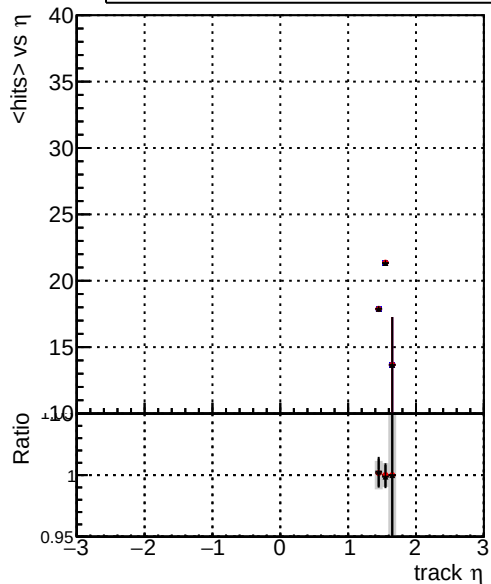
mean hits — DQM_original_step2_pt1to1000_eta1p4to1p6 — DQM_mkFit_step2_pt1to1000_eta1p4to1p6 — DQM_pixelCPETemplate_step2_pt1to1000_eta1p4to1p6
